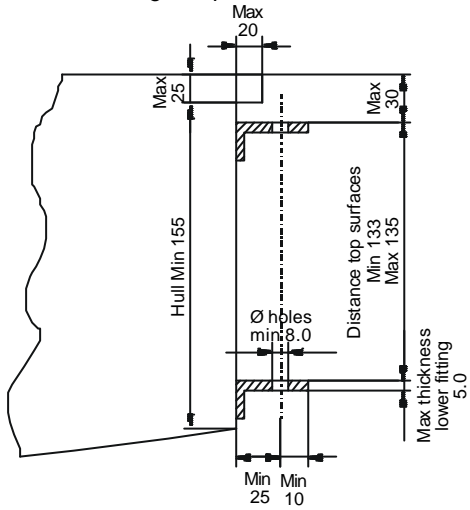
Rudder Fittings Replacement Measurement Diagram
